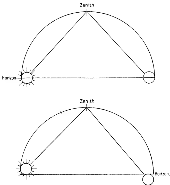
Fig. 39. Sun, moon, and zenith.
